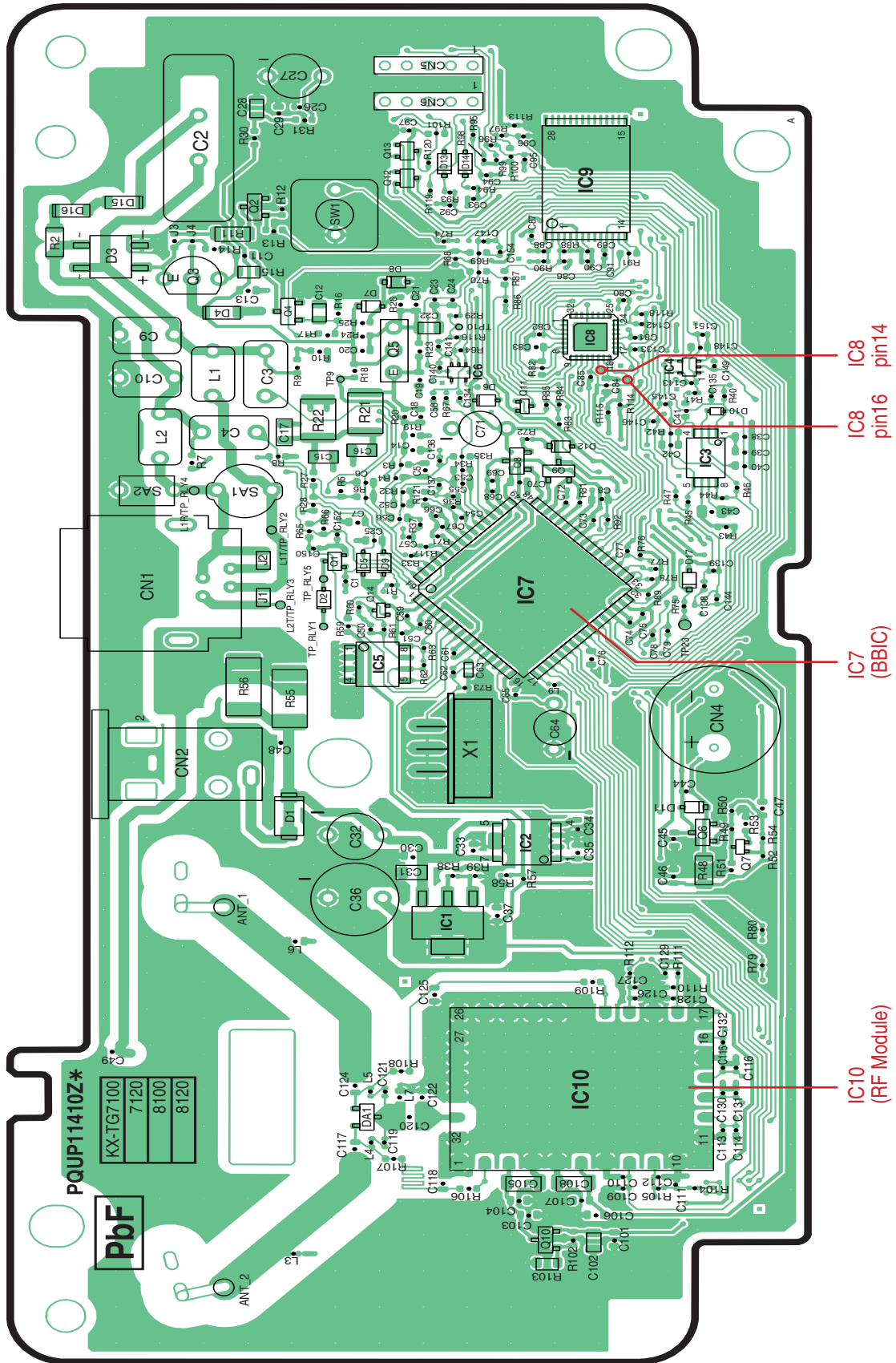
KX-TG7100/7102/7103 CIRCUIT BOARD (Base Unit (Component View))
