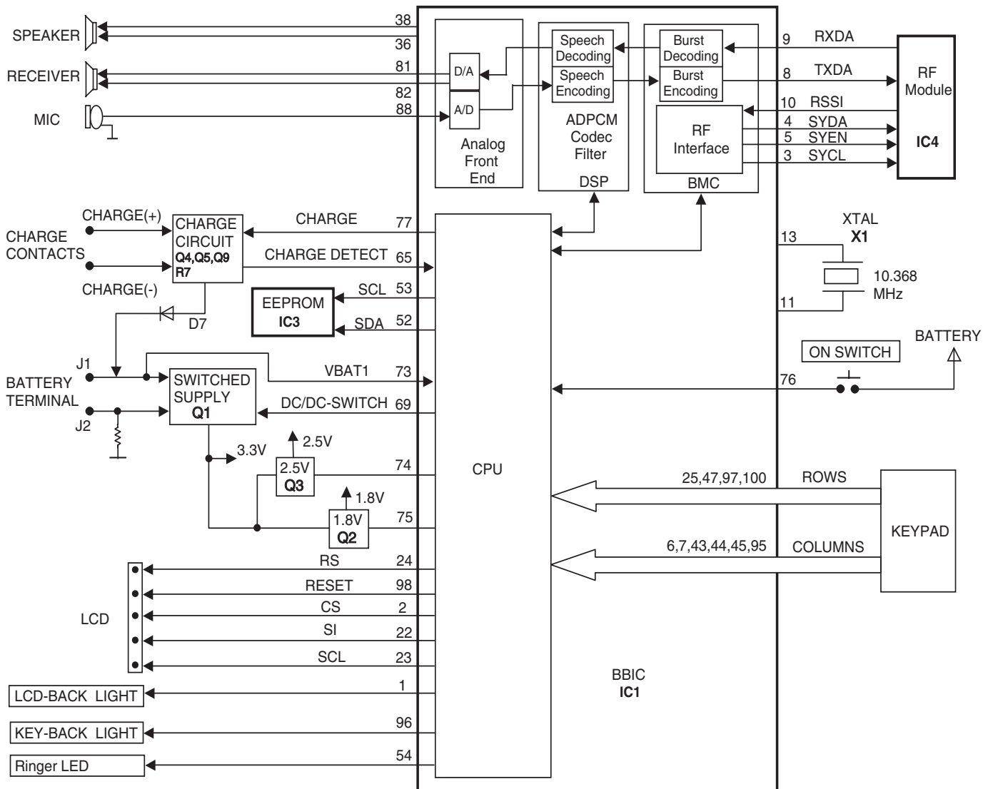
KX-TGA710 BLOCK DIAGRAM (HANDSET)
