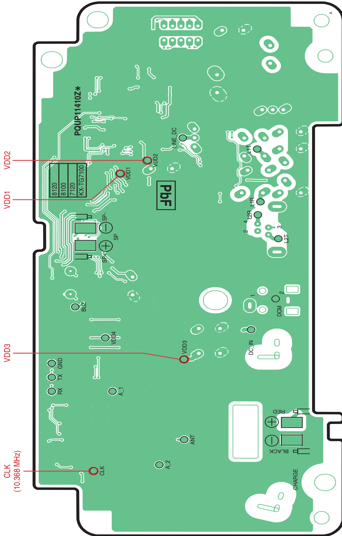
KX-TG7100/7102/7103 CIRCUIT BOARD (Base Unit (Flow Solder Side View))
