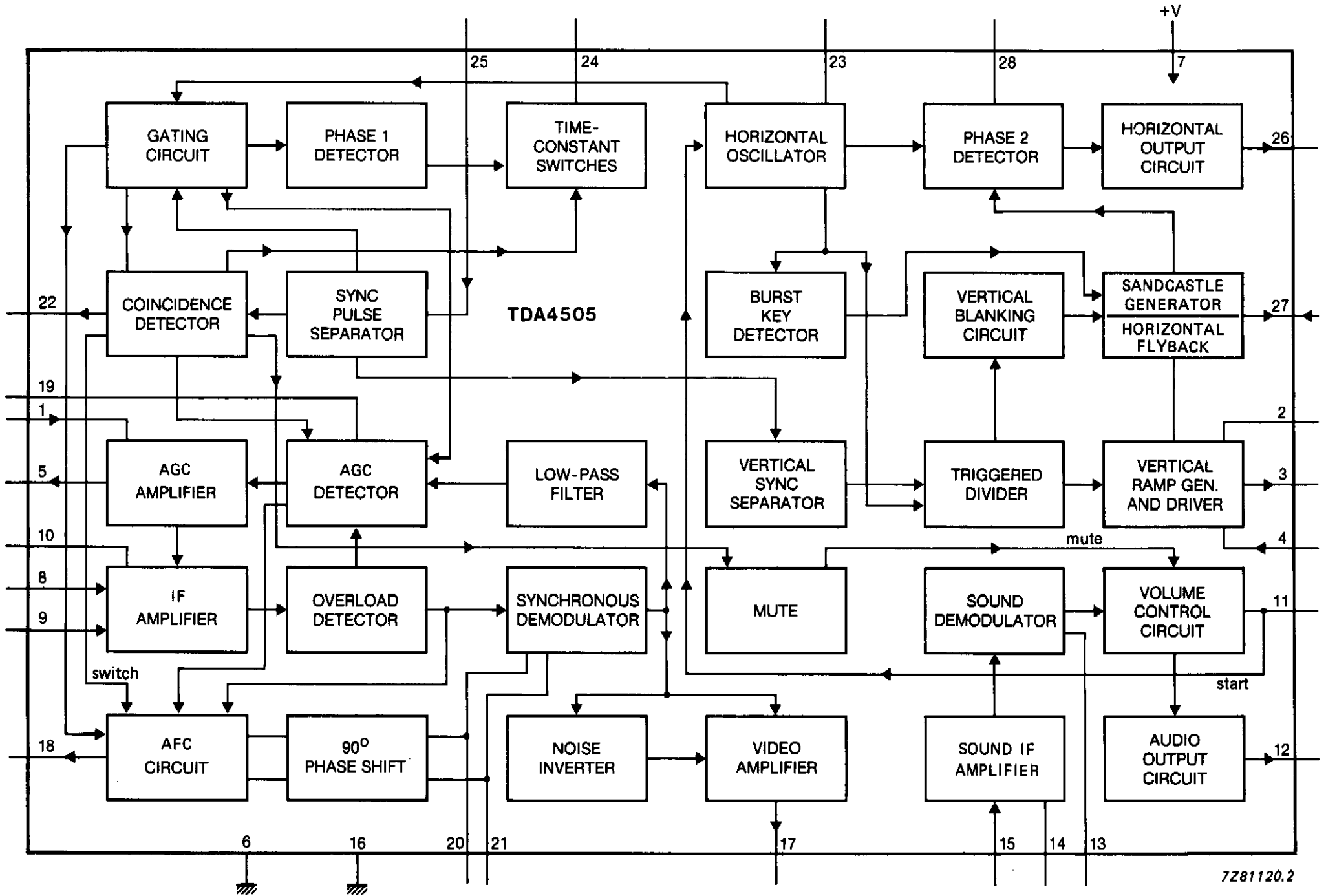
Fig. 1 Block diagram.
