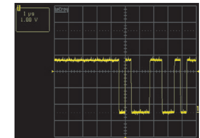
3 OPEN, CLOSE WAVEFORM ZIC1 Pin(99,102), MIC1(9,10)
