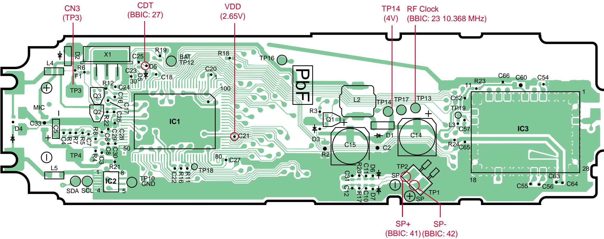
KX-TCD410ES CIRCUIT BOARD (HANDSET) Component View
